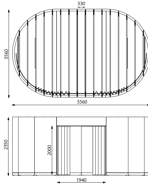
BuildUp Meeting Pod R8 (17 m 2 , 8-10 persons)
