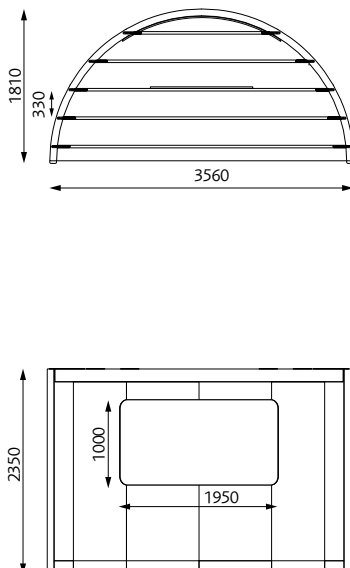
BuildUp Meeting Pavilion R4 (5 m 2 , 4-6 persons)
