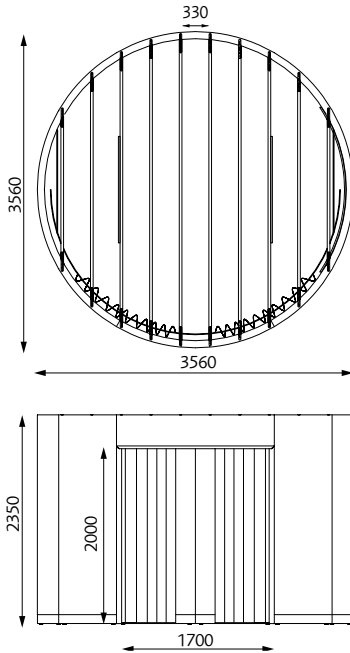
BuildUp Meeting Pod R4 (10 m 2 , 4-6 persons)
