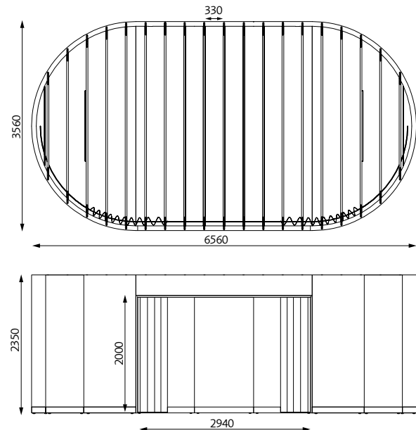
BuildUp Meeting Pod R12 (20 m 2 , 12-14 persons)
